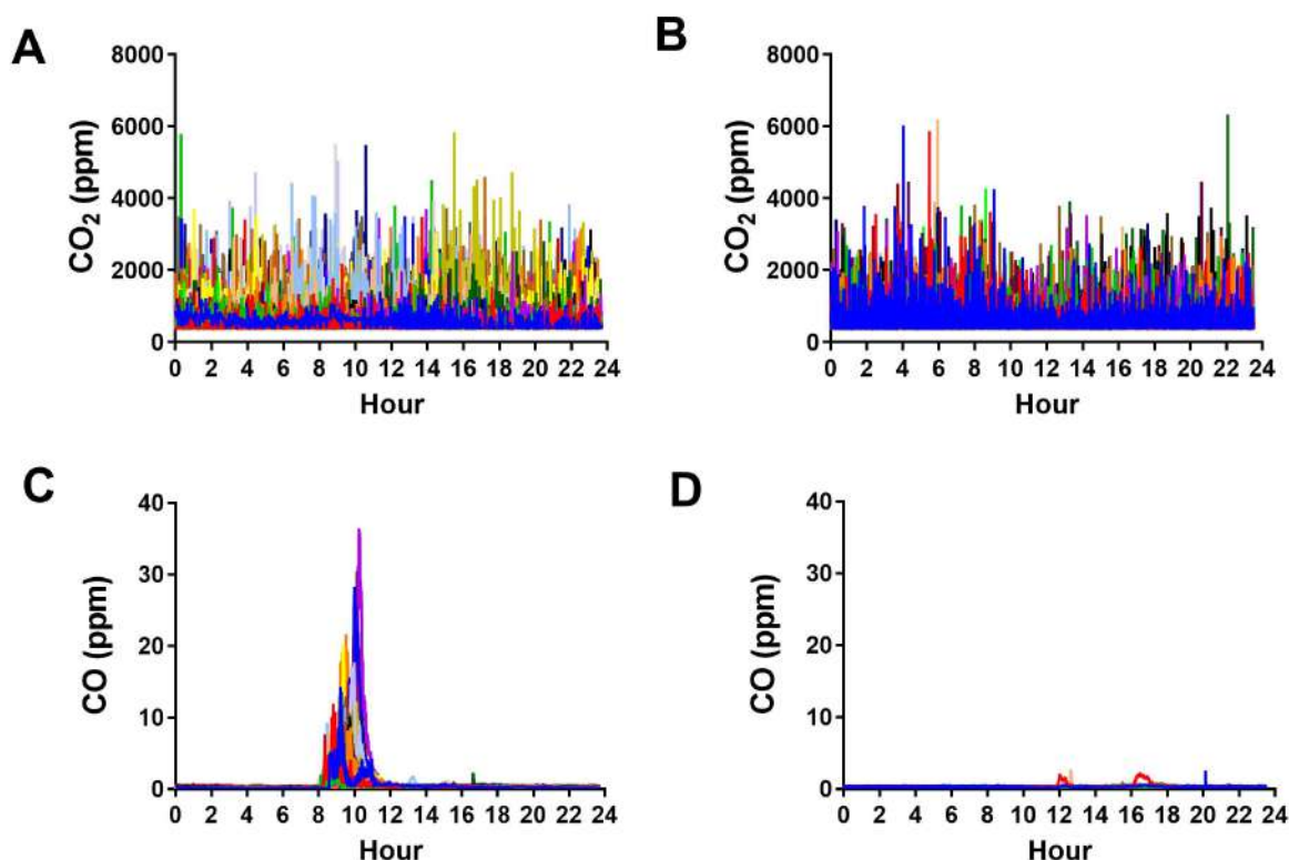
Figure 3: Carbon dioxide ( \text{CO}_2 ) and Carbon monoxide (CO) of Yagya fumes in an open room setting. Left Panel A and C, represent Carbon dioxide ( \text{CO}_2 ) and Carbon monoxide (CO) in Yagya fumes in open room settings ( n = 40 ); fire is lit between 8 and 10 hours; right Panel B and D represent Carbon dioxide ( \text{CO}_2 ) and Carbon monoxide (CO) of normal air (without Yagya) in the same open room settings ( n = 14 )
