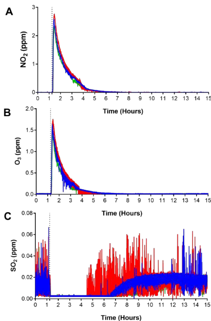
Figure 6: Nitrogen oxide ( \text{NO}_2 ), ozone ( \text{O}_3 ), and sulfur dioxide ( \text{SO}_2 ) of wood, ghee, and hawan samagri (W+G+H) in a closed-room setting. A, B, and C represent \text{NO}_2 , \text{O}_3 , and \text{SO}_2 , respectively, of W+G+H fumes in closed-room settings ( n = 3 ); the dotted line at 1.25 hours indicates the start of the fire in the closed room.
